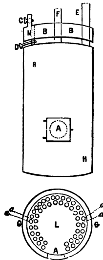
FIG. 74.—Read's Multi-Tubular Boiler, 1788.
